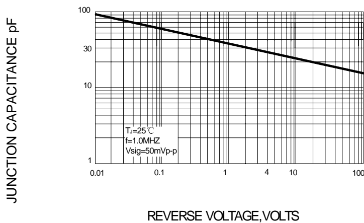
FIG.5-TYPICAL JUNCTION CAPACITANCE
